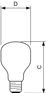
STD SOFT 60W E27 240V T55 SW
